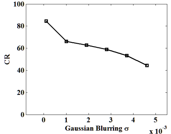
Fig. 9. Correct ratio per Gaussian Blurring Sigma
