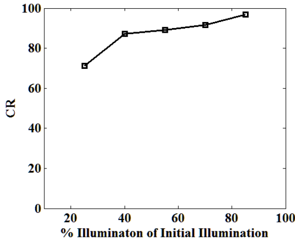
Fig. 7. Correct ratio per Illumination Changes.
