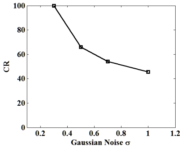
Fig. 8. Correct ratio per Gaussian Noise Sigma.
